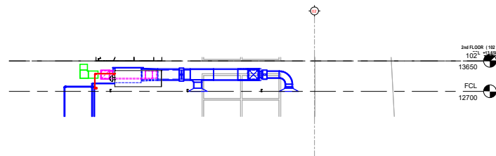
① Section VIEW OF HVAC 1 : 50
