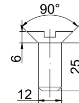
Set screw (1 no- MS)
