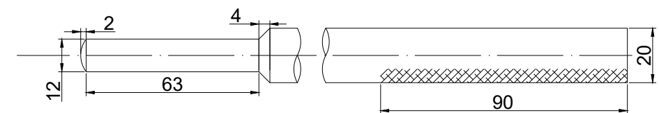
Tommy Bar(1 No -MS)
