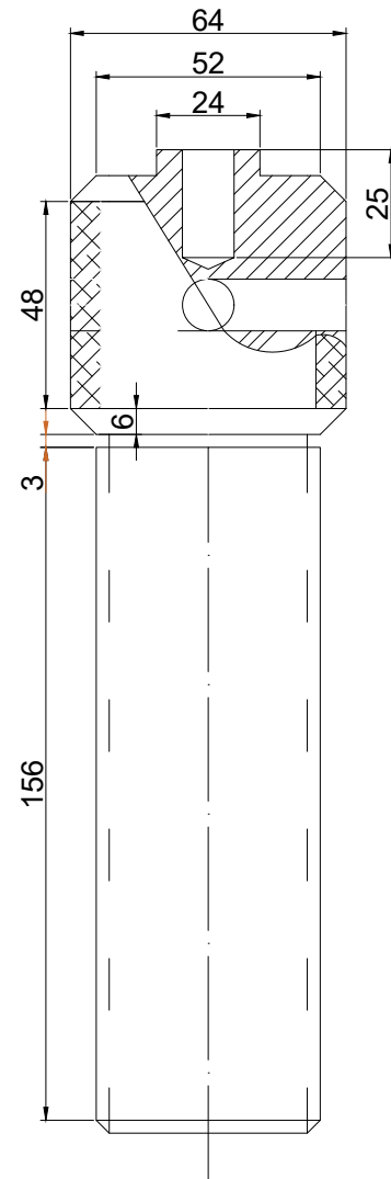
screw rod (1 no- MS)
